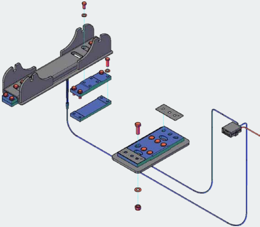
Illustration diagram of Mixer Scales setup
